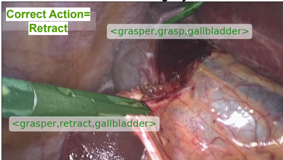
Action Ambiguity
