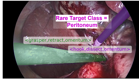
Rare Classes
