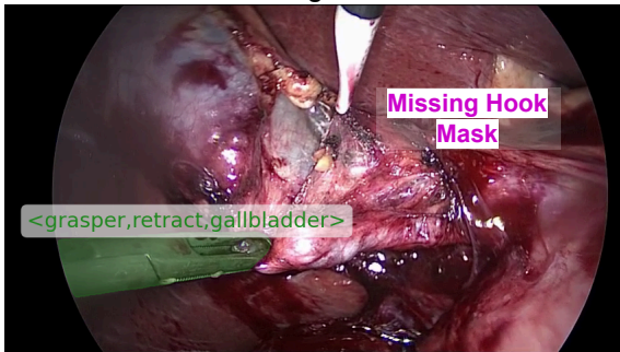
Missing Mask
